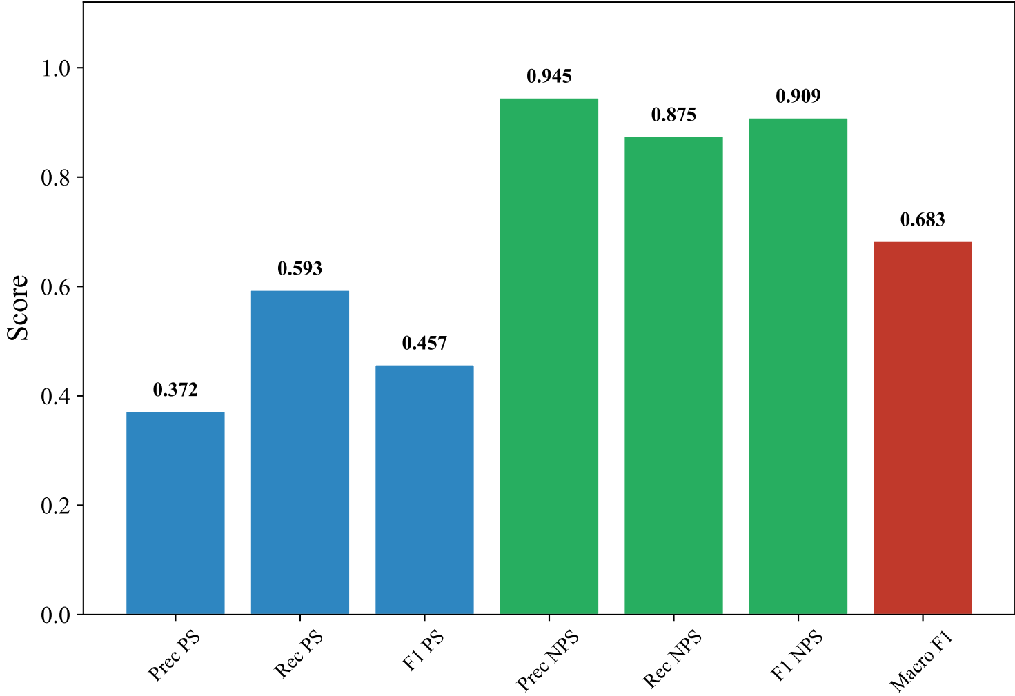
Classification Metrics — GERMAN_MANUAL (efederici/e5-base-multilingual-4096, LightGBM)
