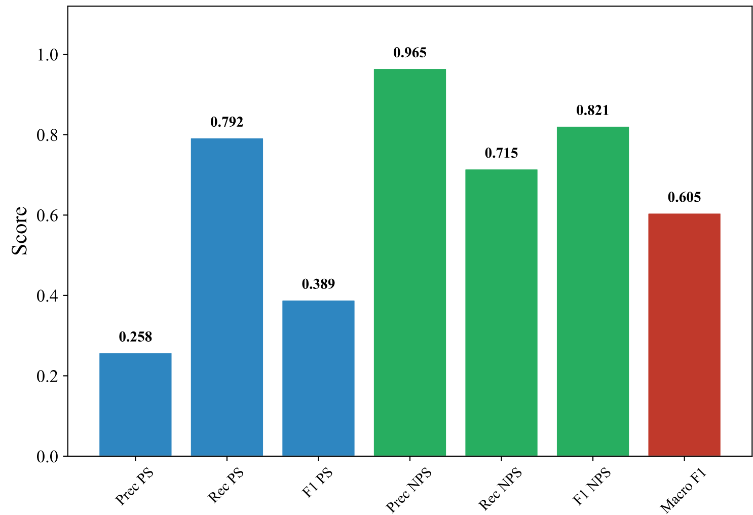
Classification Metrics — GERMAN_MANUAL (intfloat/multilingual-e5-large-instruct, Random_Forest)
