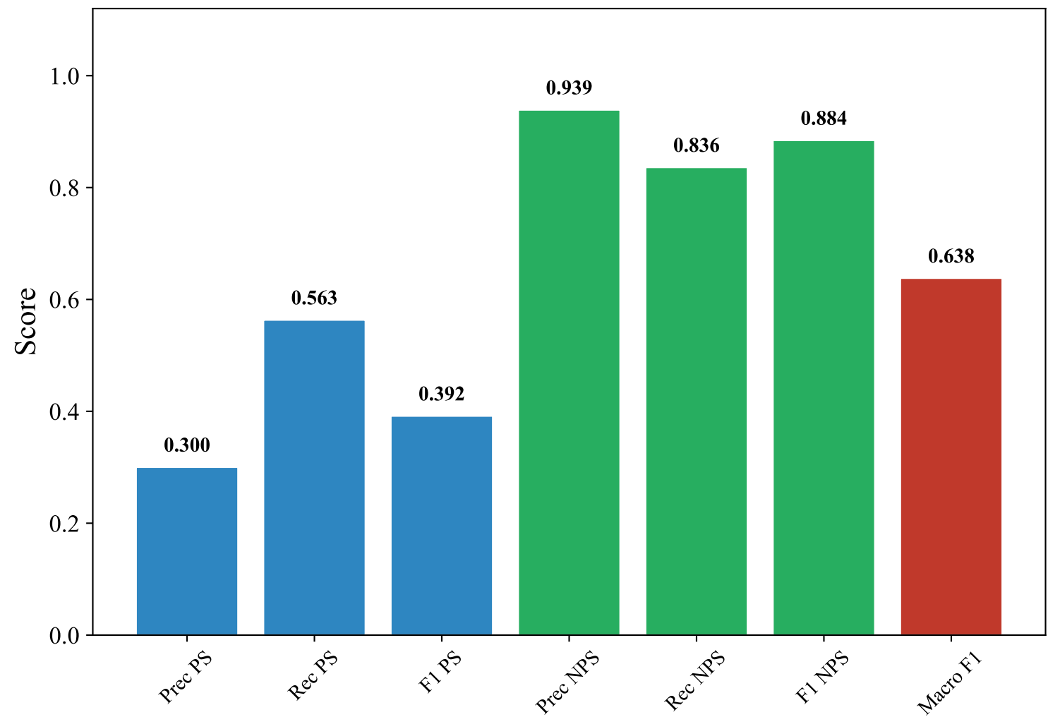
Classification Metrics — GERMAN_MANUAL (paraphrase-multilingual-MiniLM-L12-v2, XGBoost)
