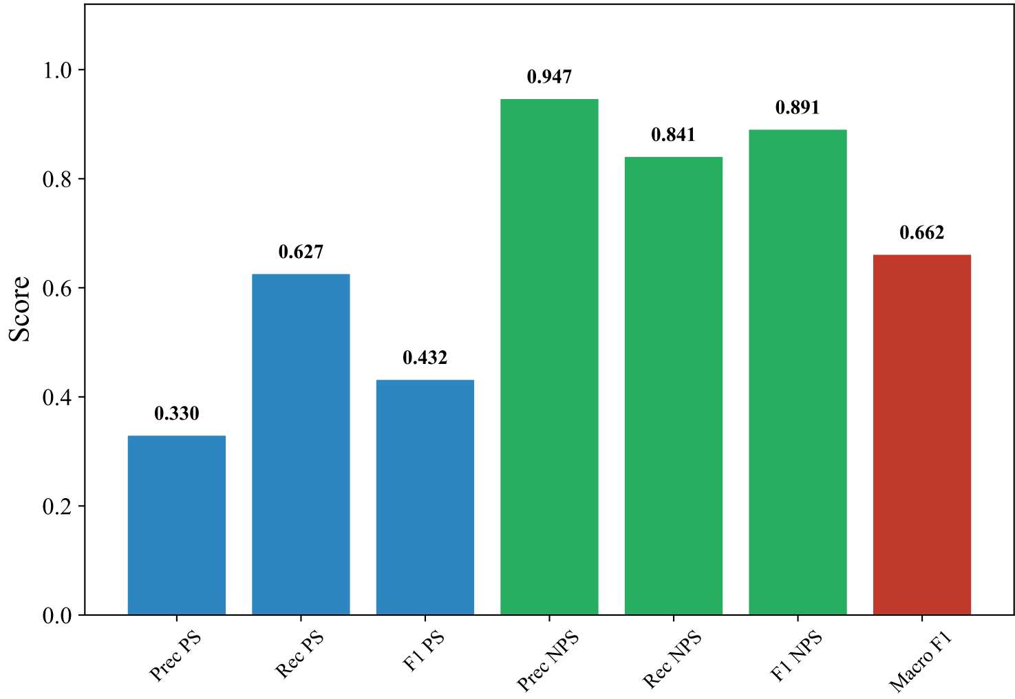
Classification Metrics — GERMAN_MANUAL (paraphrase-multilingual-mpnet-base-v2, LightGBM)
