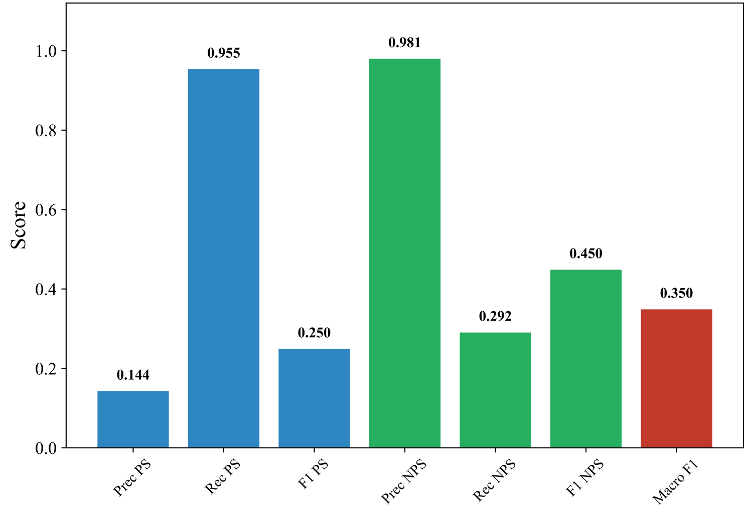
Classification Metrics — GERMAN_MANUAL (snowflake-arctic-embed-l-v2.0, Random_Forest_Optimized)
