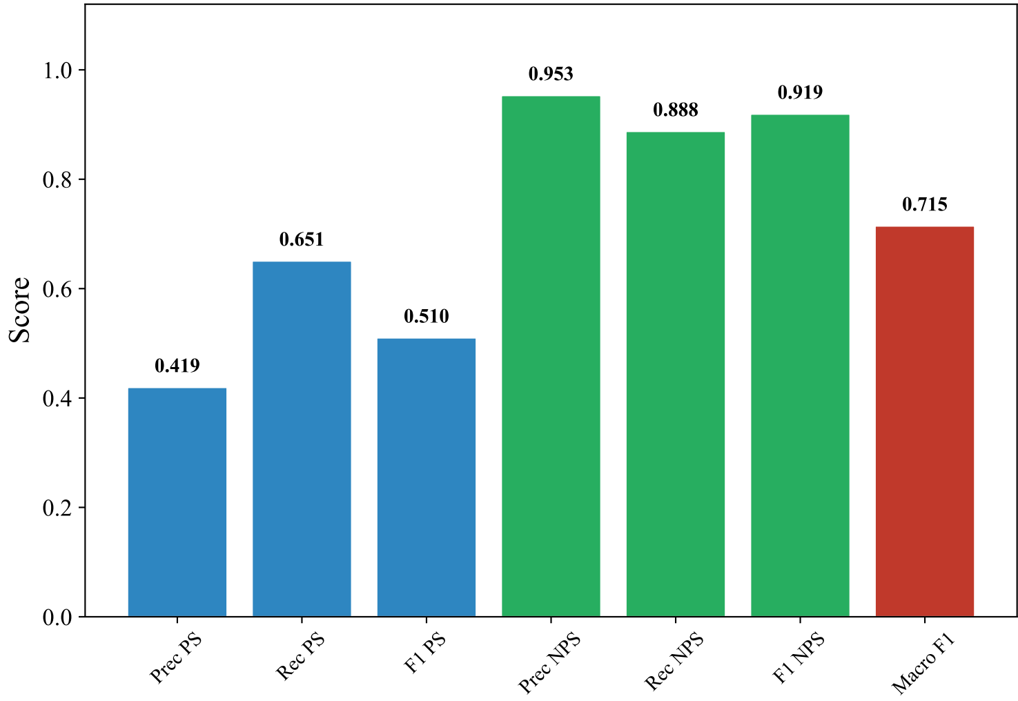
Classification Metrics — GERMAN_MANUAL (snowflake-arctic-embed-l-v2.0, XGBoost_Optimized)
