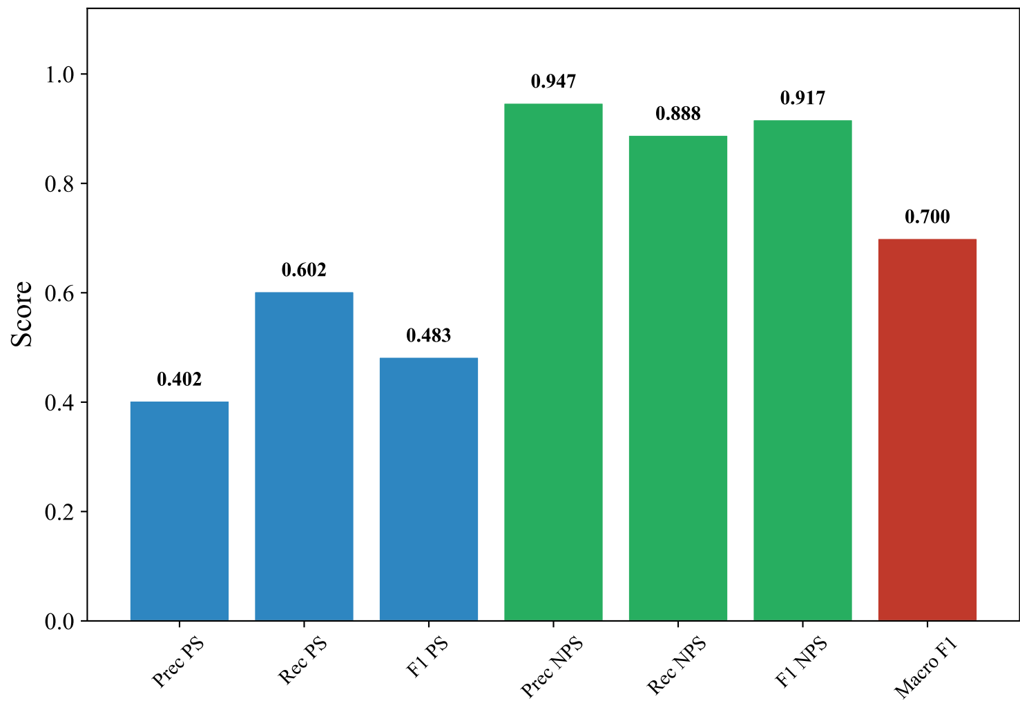
Classification Metrics — GERMAN_MANUAL (upskyy/bge-m3-korean, LightGBM)
