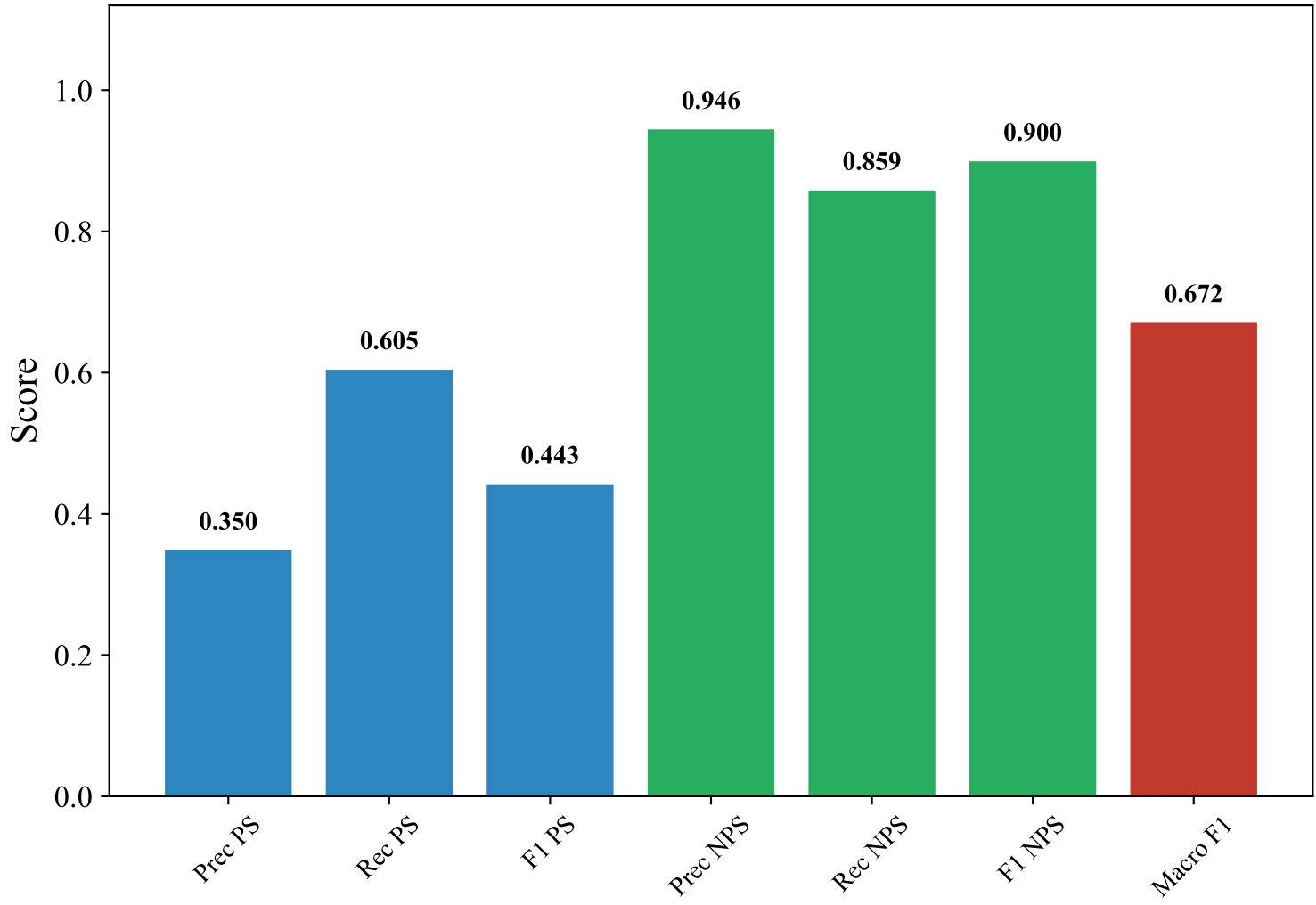
Classification Metrics — GERMAN_MANUAL (xlm-roberta-base, LightGBM)
