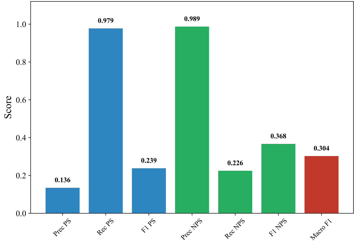
Classification Metrics — GERMAN_MANUAL (xlm-roberta-base, Random_Forest_Optimized)
