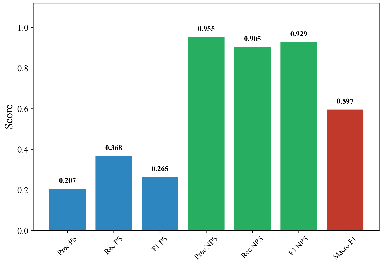
Classification Metrics — SWEDISH_MANUAL (efederici/e5-base-multilingual-4096, XGBoost_Optimized)
