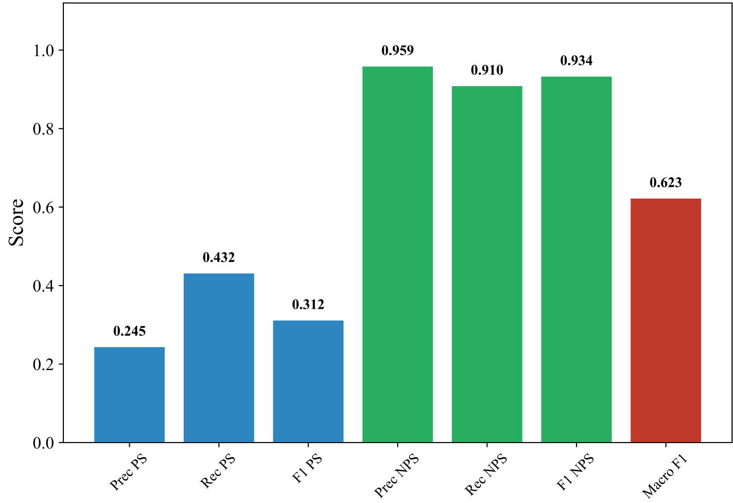
Classification Metrics — SWEDISH_MANUAL (intfloat/multilingual-e5-large-instruct, LightGBM)
