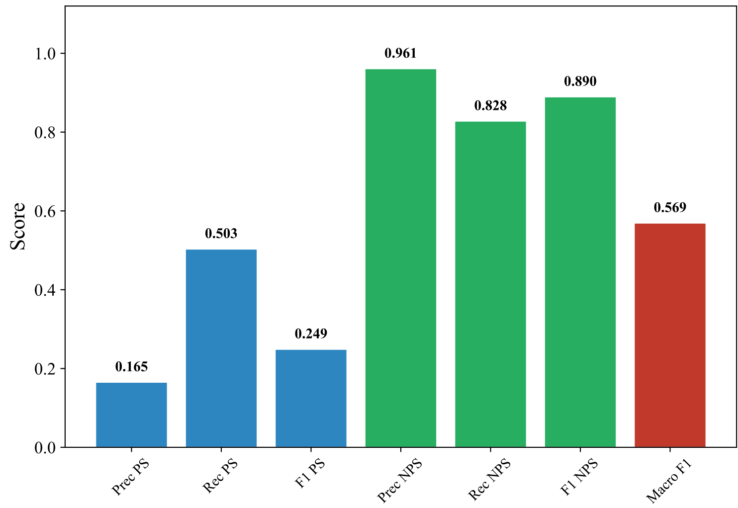
Classification Metrics — SWEDISH_MANUAL (intfloat/multilingual-e5-large-instruct, SVM)
