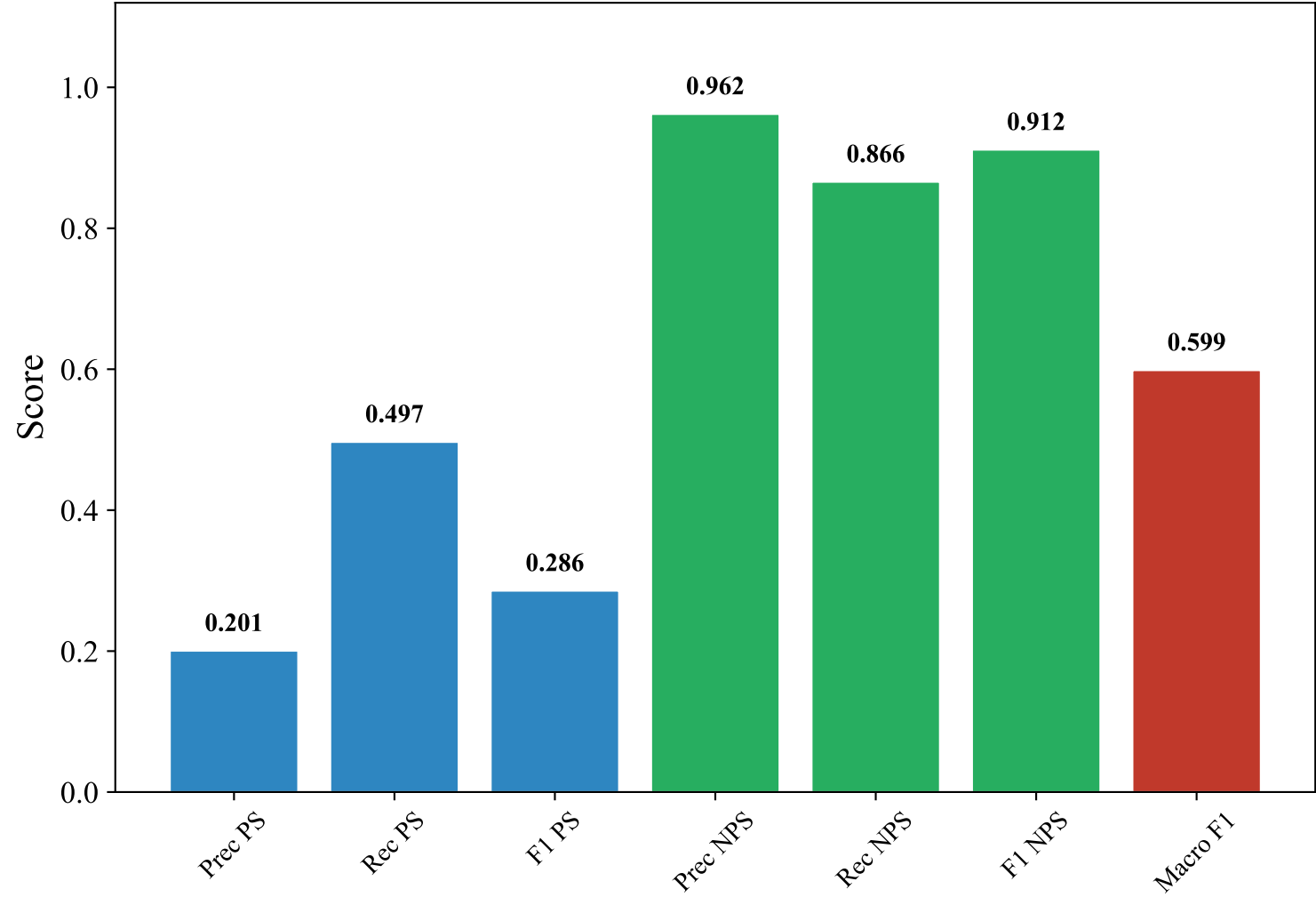
Classification Metrics — SWEDISH_MANUAL (paraphrase-multilingual-MiniLM-L12-v2, Voting_Ensemble)
