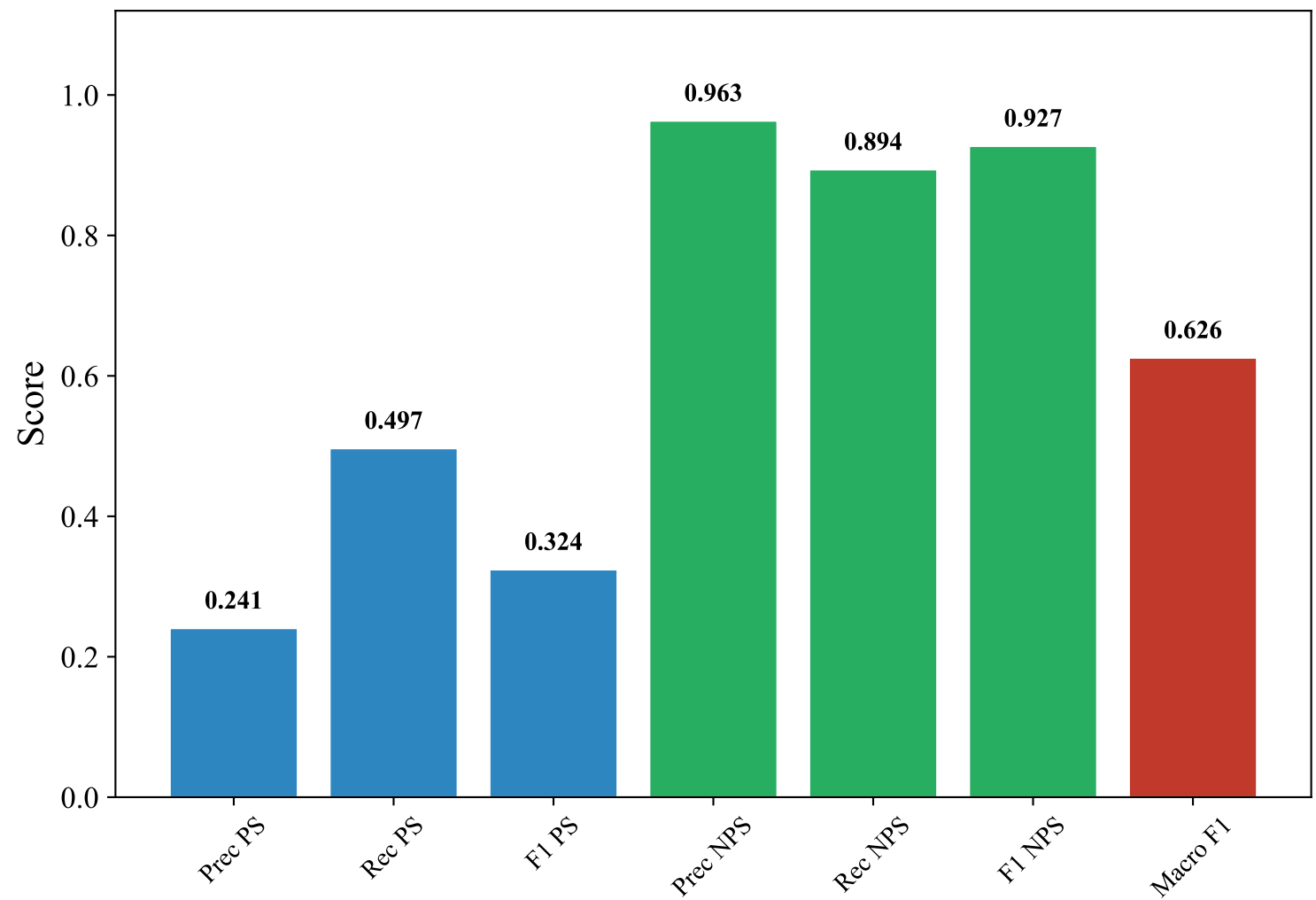
Classification Metrics — SWEDISH_MANUAL (snowflake-arctic-embed-l-v2.0, Voting_Ensemble)
