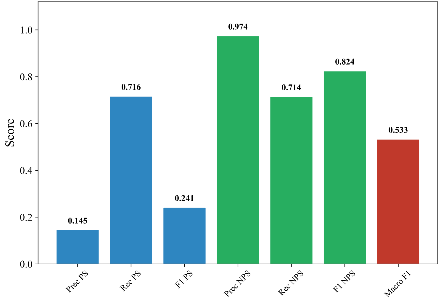
Classification Metrics — SWEDISH_MANUAL (upskyy/bge-m3-korean, Random_Forest)
