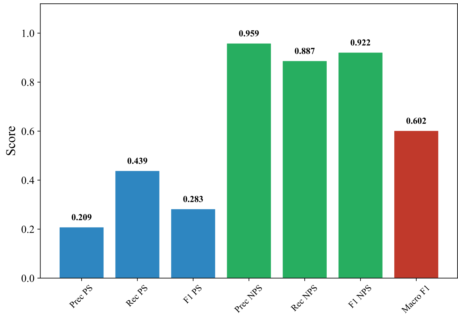
Classification Metrics — SWEDISH_MANUAL (upskyy/bge-m3-korean, Voting_Ensemble)
