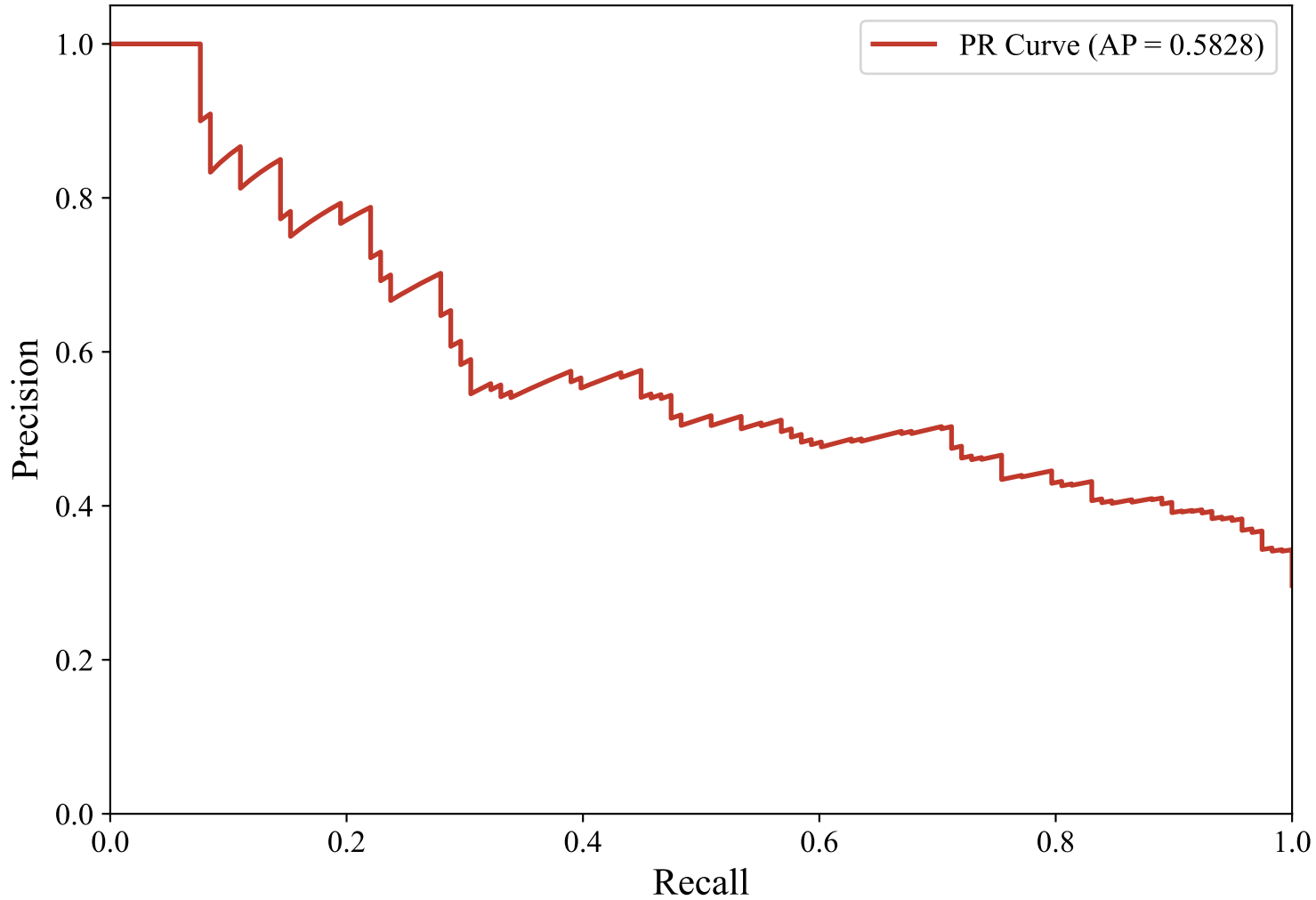
Precision-Recall Curve — DUTCH_MANUAL (bert-base-multilingual-uncased, XGBoost_Optimized)
