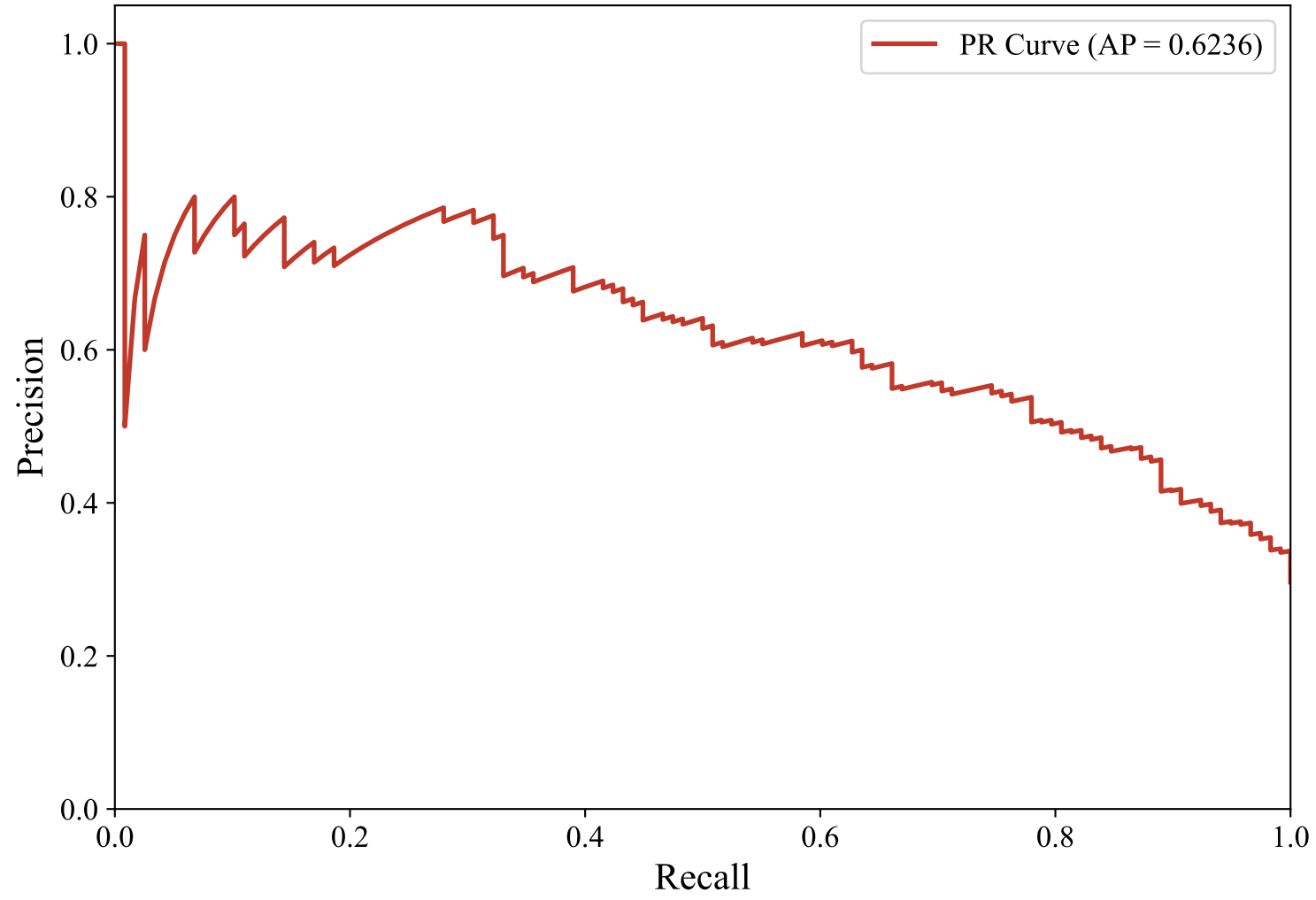
Precision-Recall Curve — DUTCH_MANUAL (efederici/e5-base-multilingual-4096, LightGBM)
