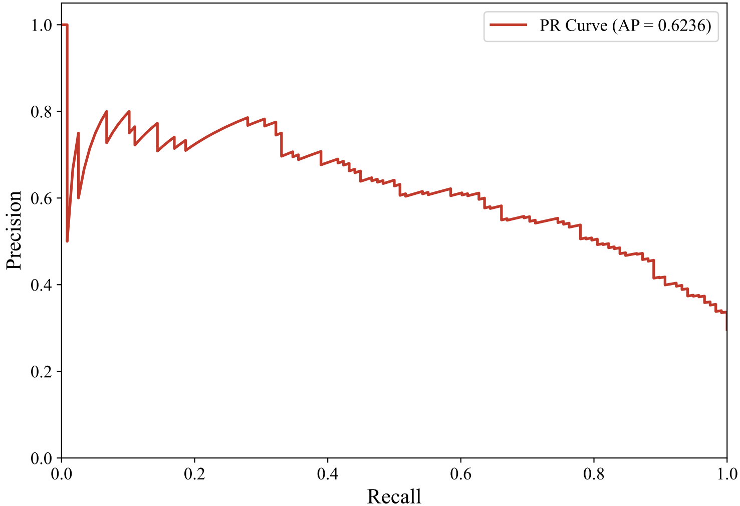
Precision-Recall Curve — DUTCH_MANUAL (efederici/e5-base-multilingual-4096, LightGBM_Optimized)
