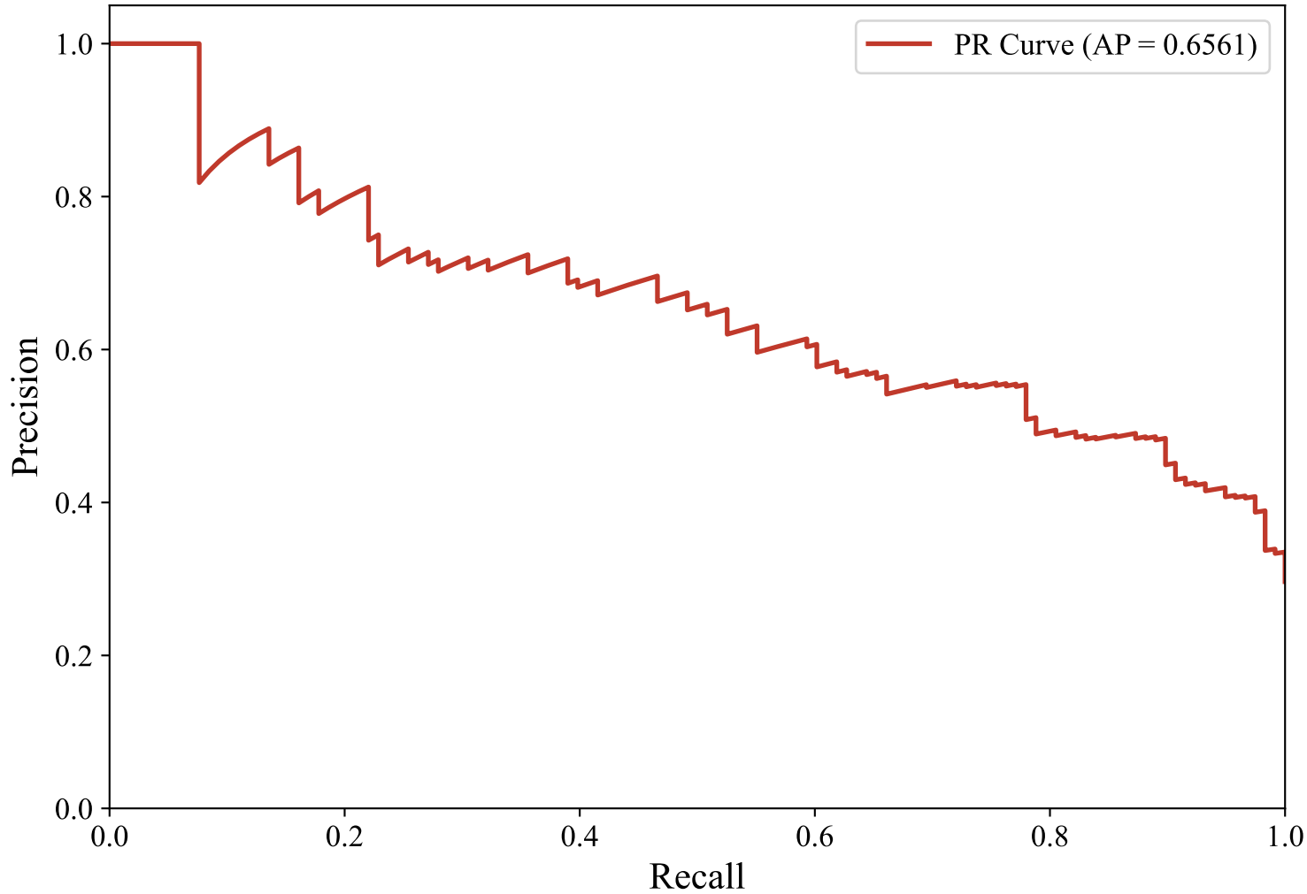
Precision-Recall Curve — DUTCH_MANUAL (efederici/e5-base-multilingual-4096, XGBoost)
