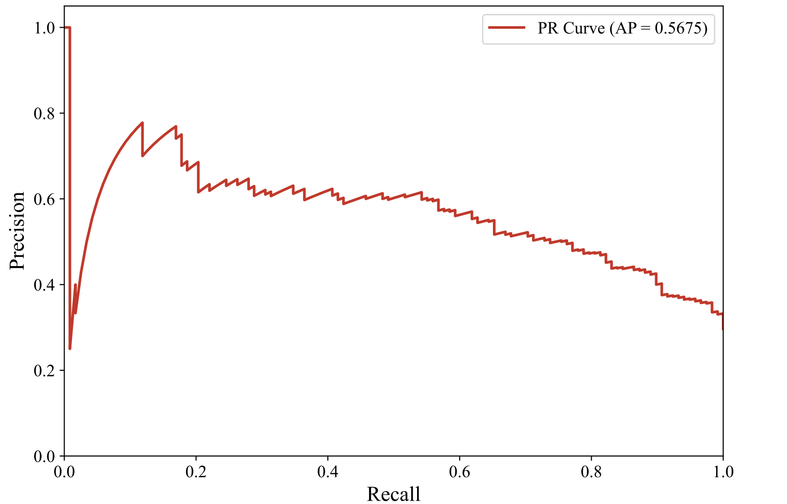
Precision-Recall Curve — DUTCH_MANUAL (paraphrase-multilingual-MiniLM-L12-v2, LightGBM)
