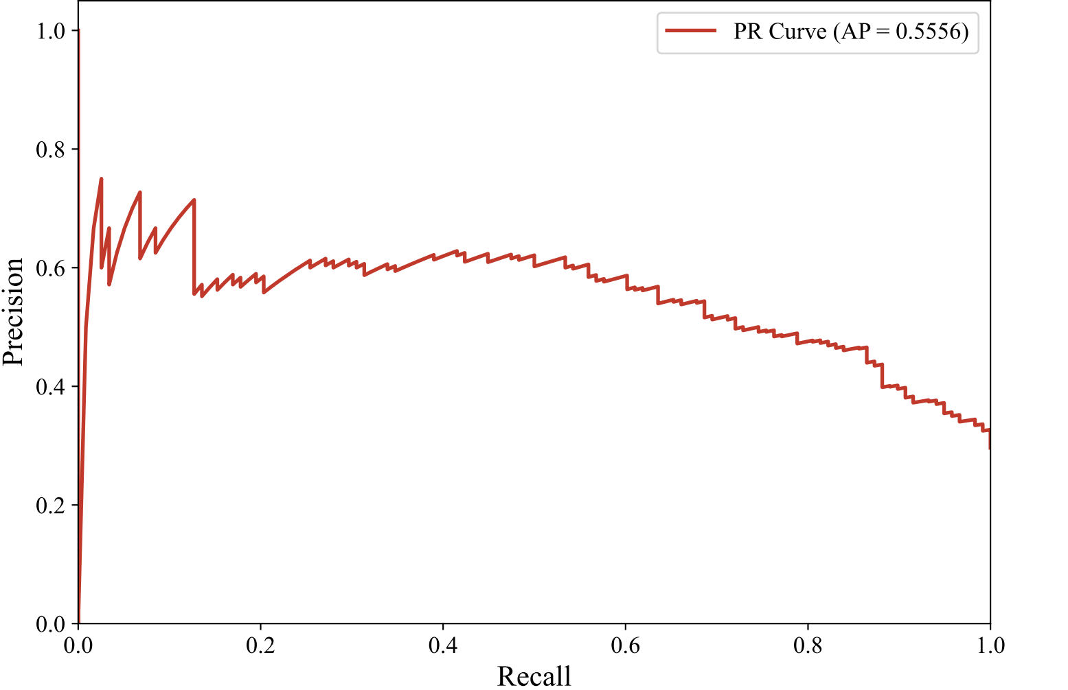
Precision-Recall Curve — DUTCH_MANUAL (paraphrase-multilingual-MiniLM-L12-v2, Voting_Ensemble)
