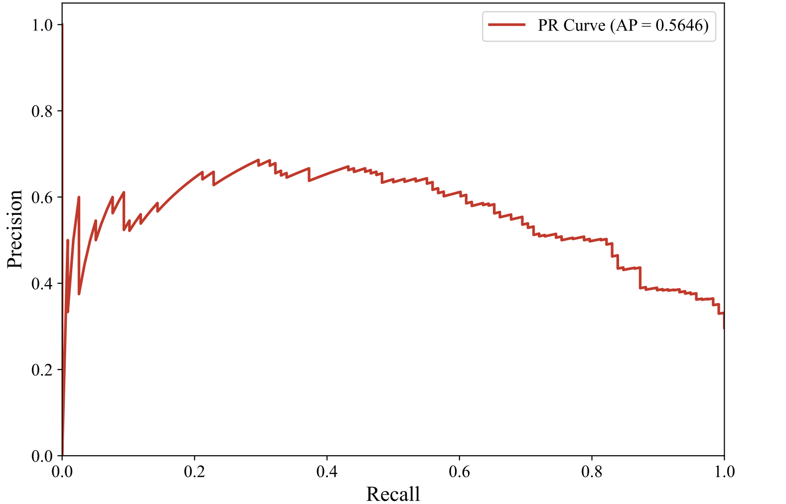
Precision-Recall Curve — DUTCH_MANUAL (paraphrase-multilingual-MiniLM-L12-v2, XGBoost)
