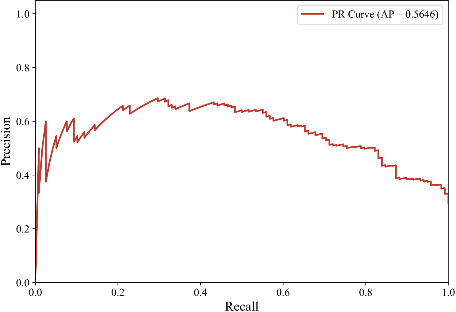
Precision-Recall Curve — DUTCH_MANUAL (paraphrase-multilingual-MiniLM-L12-v2, XGBoost_Optimized)
