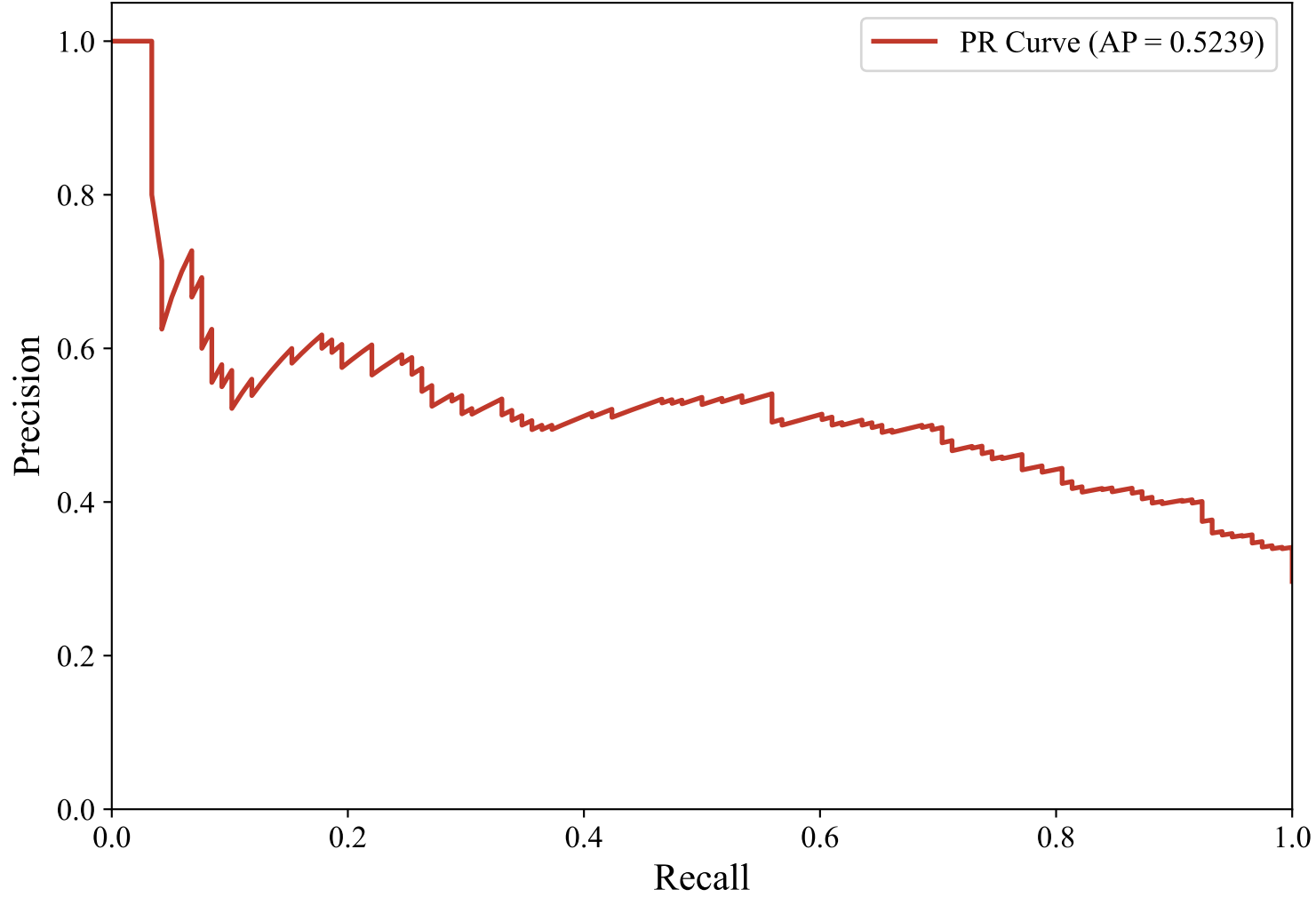
Precision-Recall Curve — DUTCH_MANUAL (paraphrase-multilingual-mpnet-base-v2, Random_Forest_Optimized)
