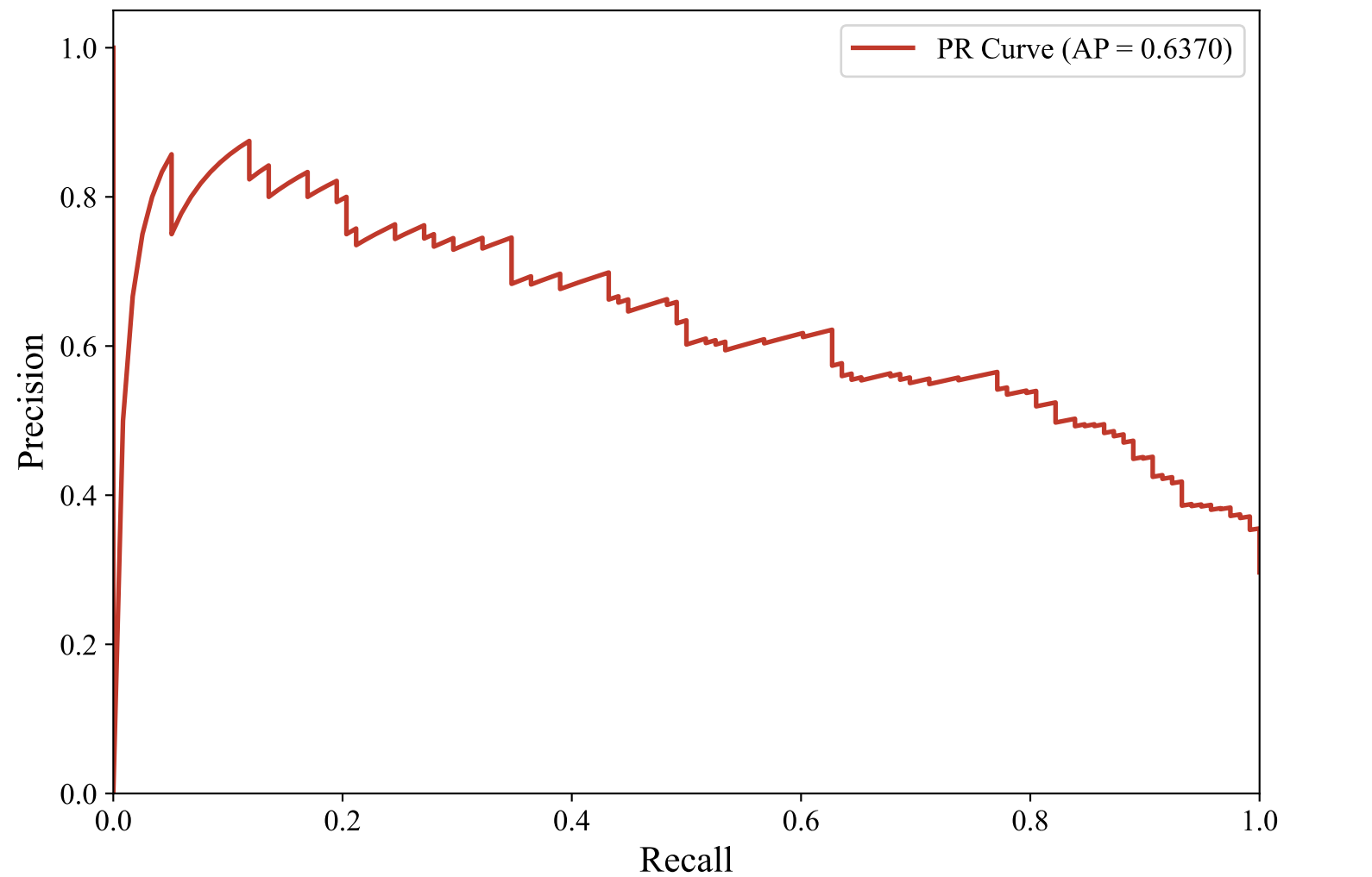
Precision-Recall Curve — DUTCH_MANUAL (snowflake-arctic-embed-l-v2.0, LightGBM_Optimized)
