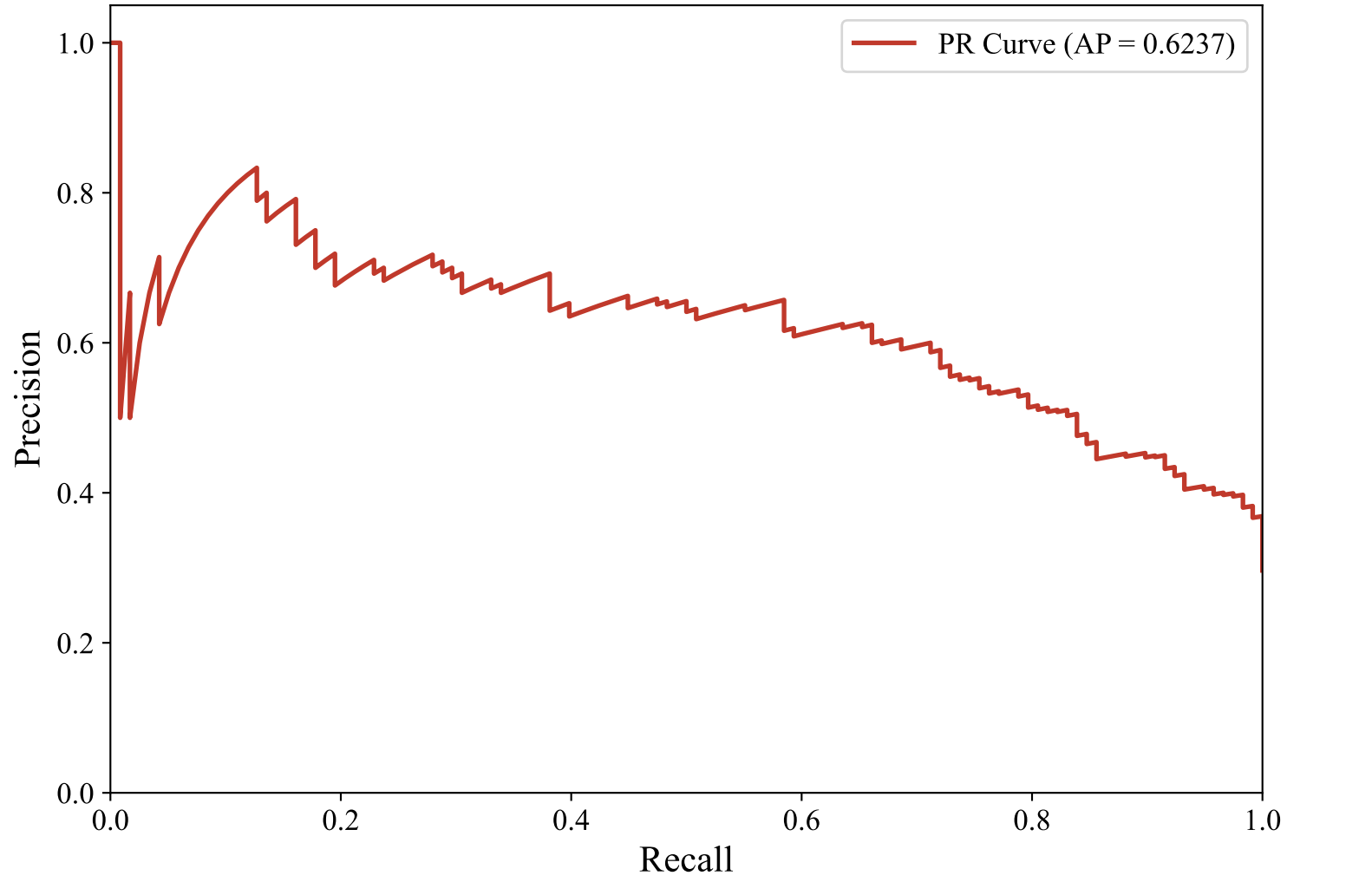
Precision-Recall Curve — DUTCH_MANUAL (snowflake-arctic-embed-l-v2.0, XGBoost_Optimized)
