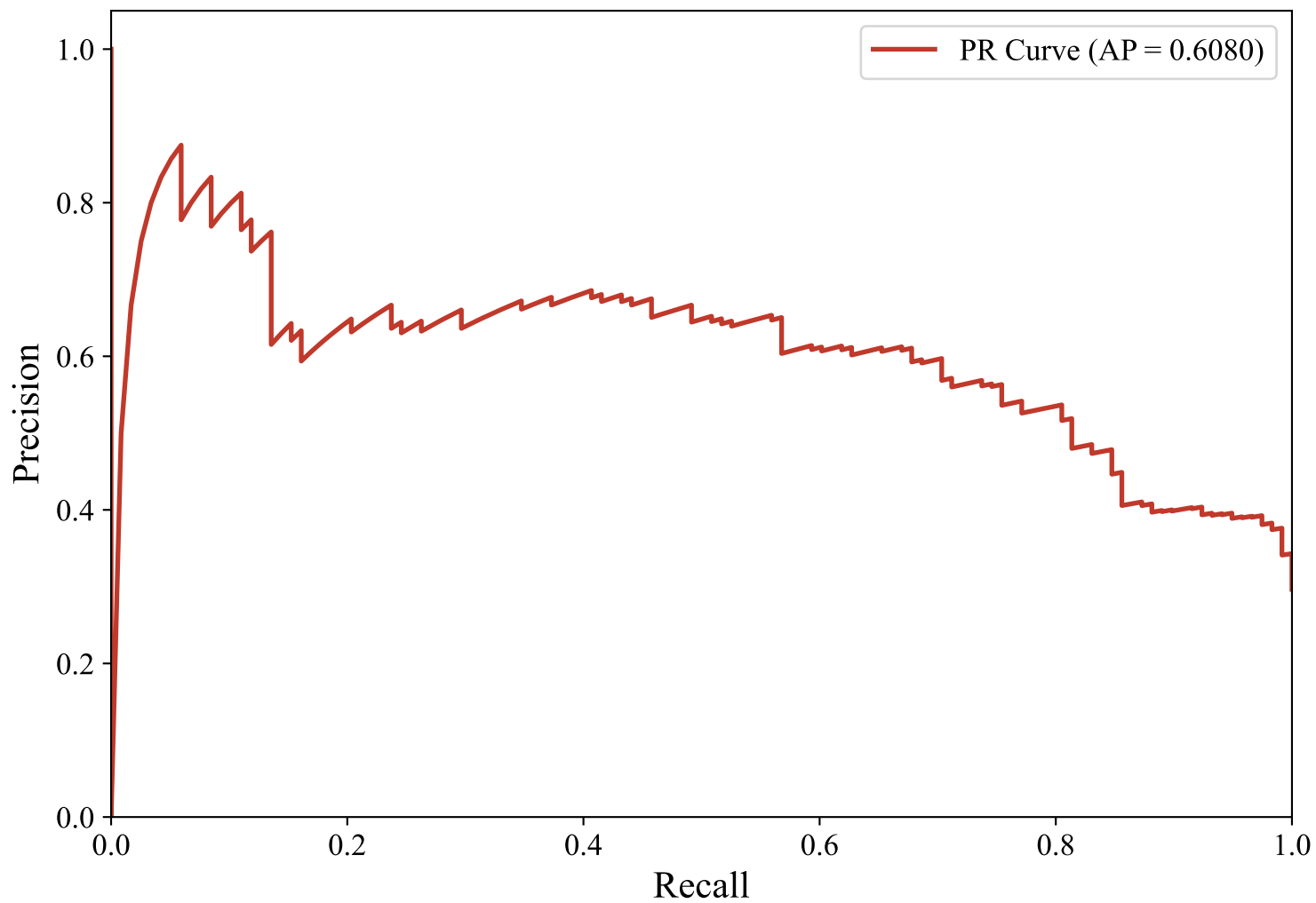
Precision-Recall Curve — DUTCH_MANUAL (xlm-roberta-base, Voting_Ensemble)
