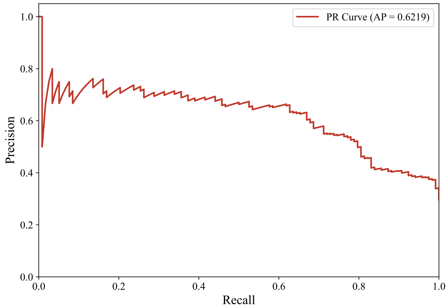
Precision-Recall Curve — DUTCH_MANUAL (xlm-roberta-base, XGBoost_Optimized)
