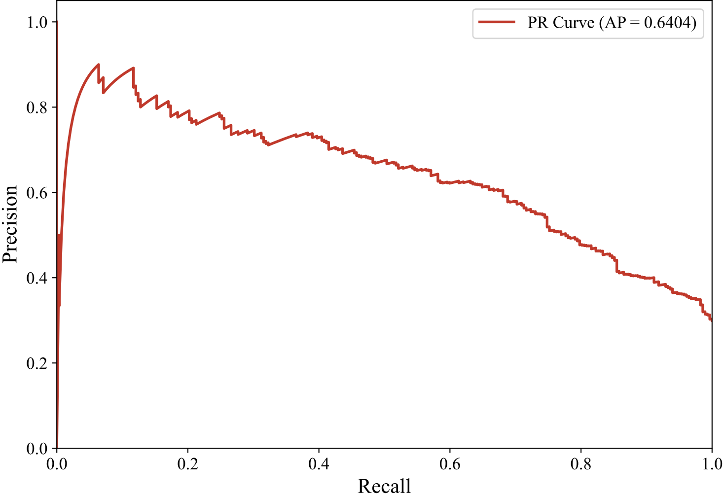
Precision-Recall Curve — ENGLISH_MANUAL (bert-base-multilingual-uncased, Random_Forest_Optimized)
