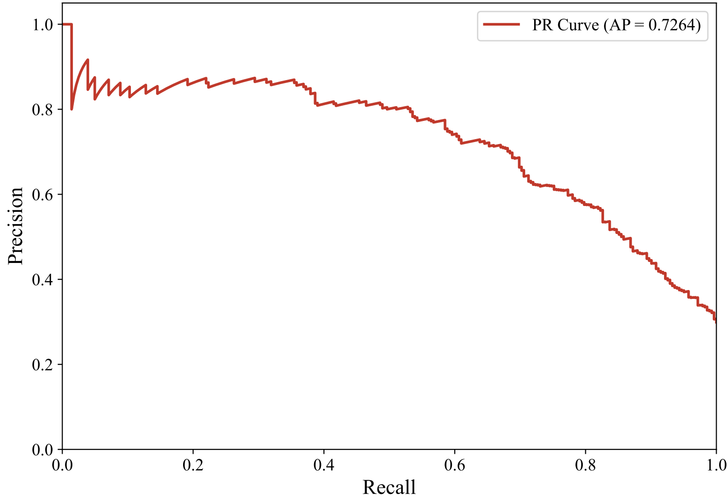
Precision-Recall Curve — ENGLISH_MANUAL (efederici/e5-base-multilingual-4096, LightGBM)
