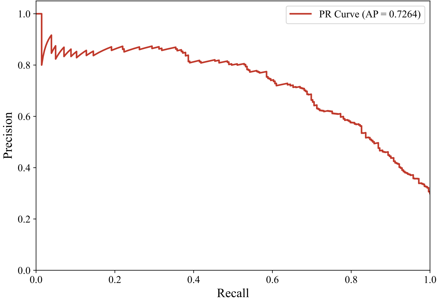
Precision-Recall Curve — ENGLISH_MANUAL (efederici/e5-base-multilingual-4096, LightGBM_Optimized)
