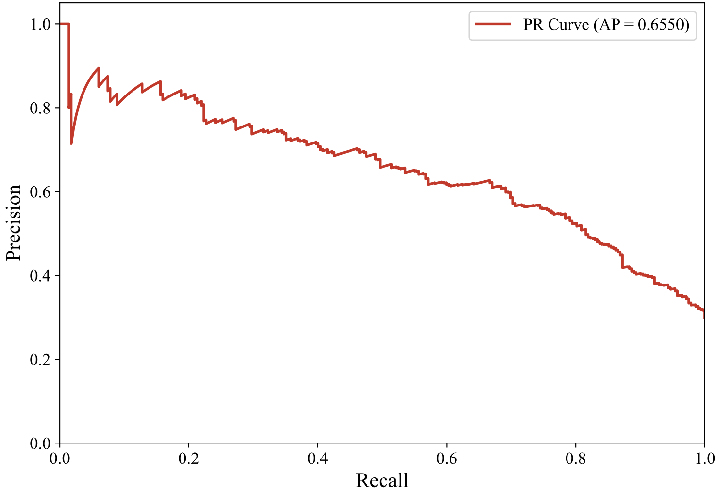
Precision-Recall Curve — ENGLISH_MANUAL (efederici/e5-base-multilingual-4096, Random_Forest)
