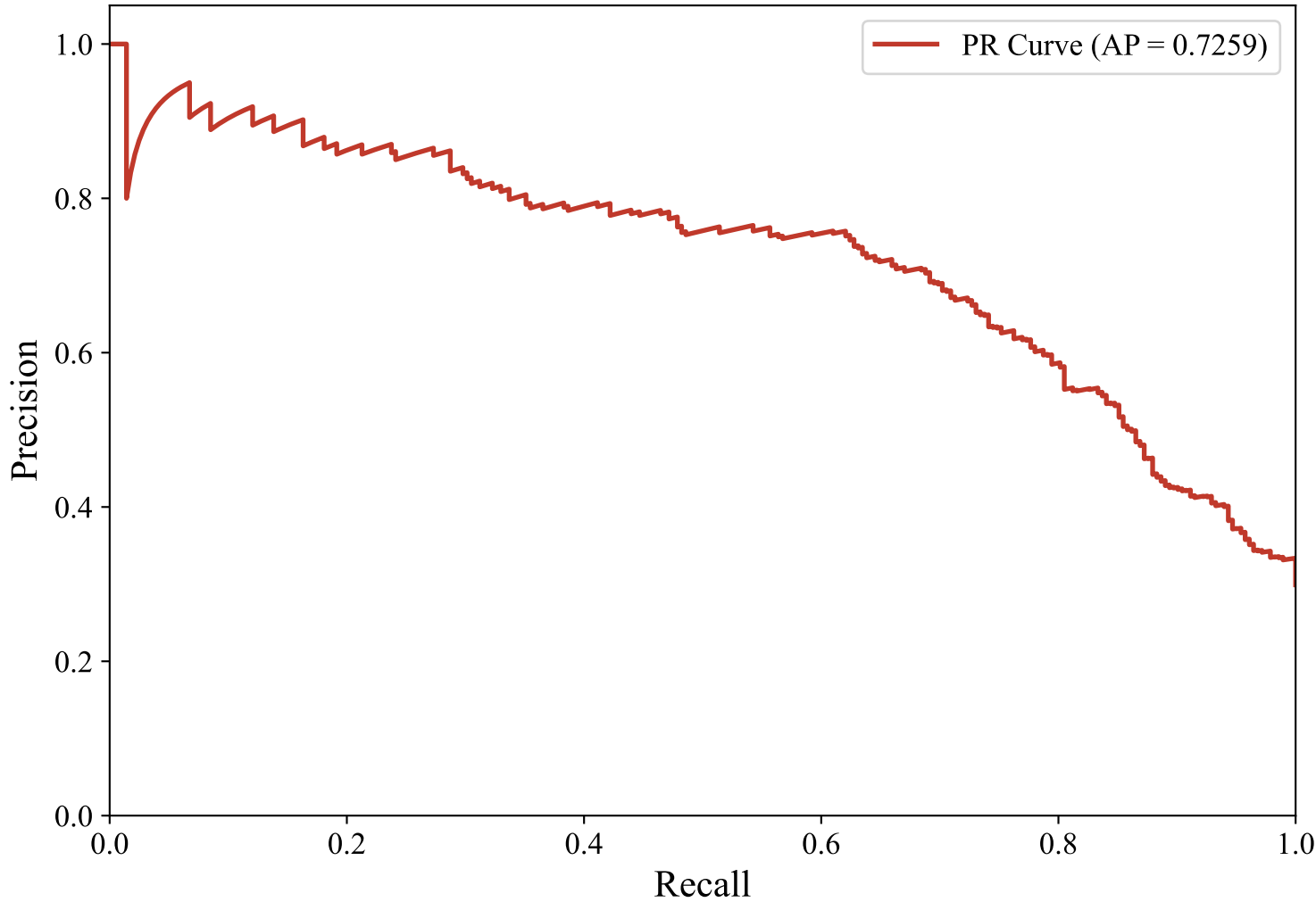
Precision-Recall Curve — ENGLISH_MANUAL (efederici/e5-base-multilingual-4096, Voting_Ensemble)
