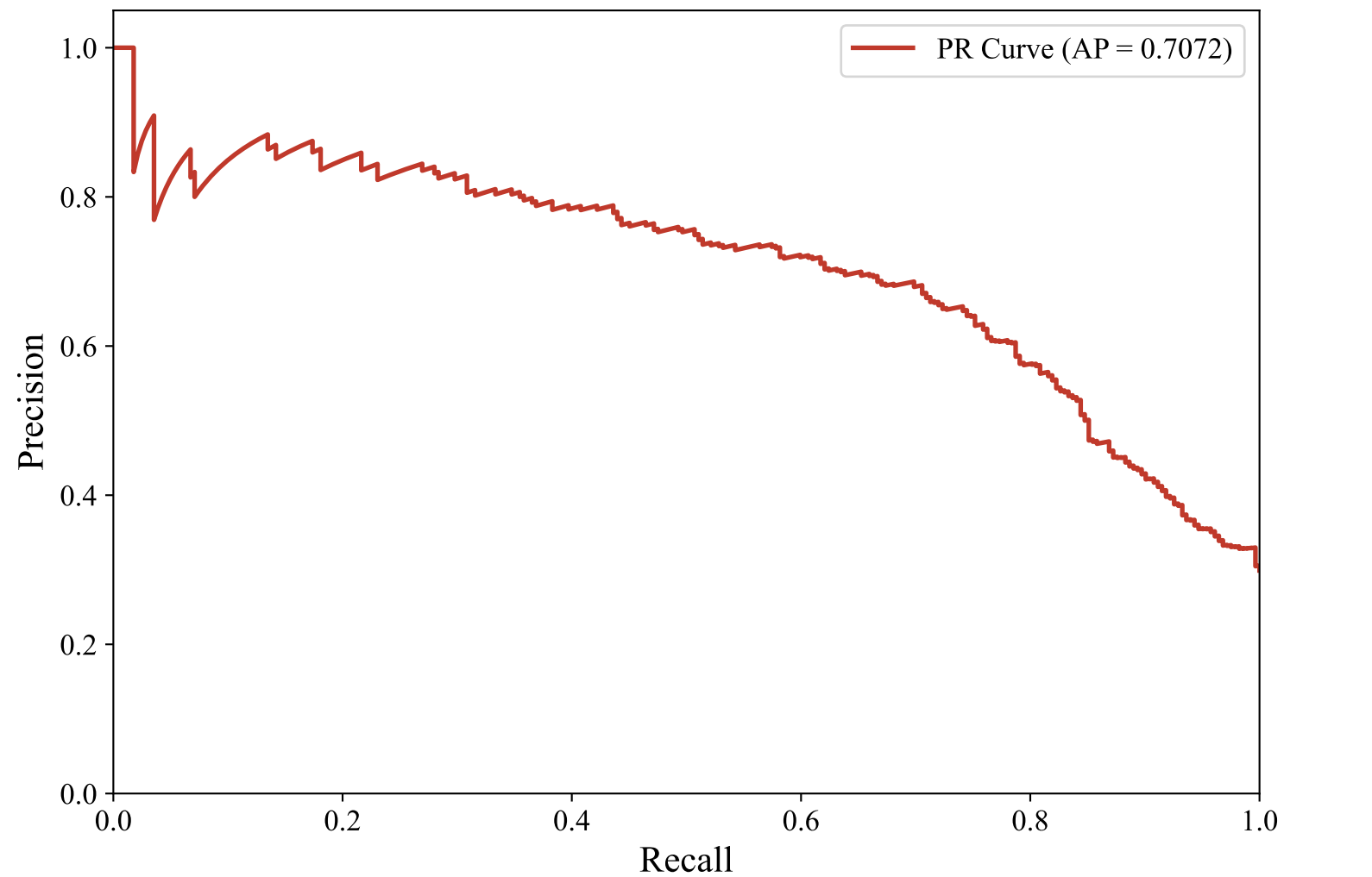
Precision-Recall Curve — ENGLISH_MANUAL (intfloat/multilingual-e5-large-instruct, Random_Forest)
