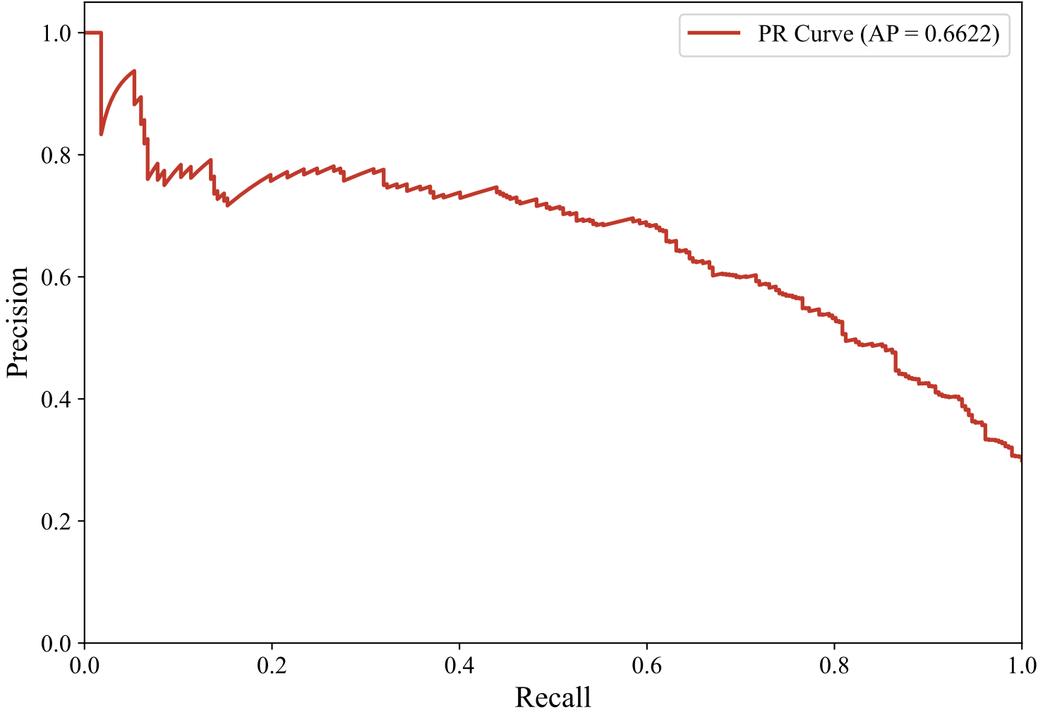
Precision-Recall Curve — ENGLISH_MANUAL (paraphrase-multilingual-MiniLM-L12-v2, Random_Forest)
