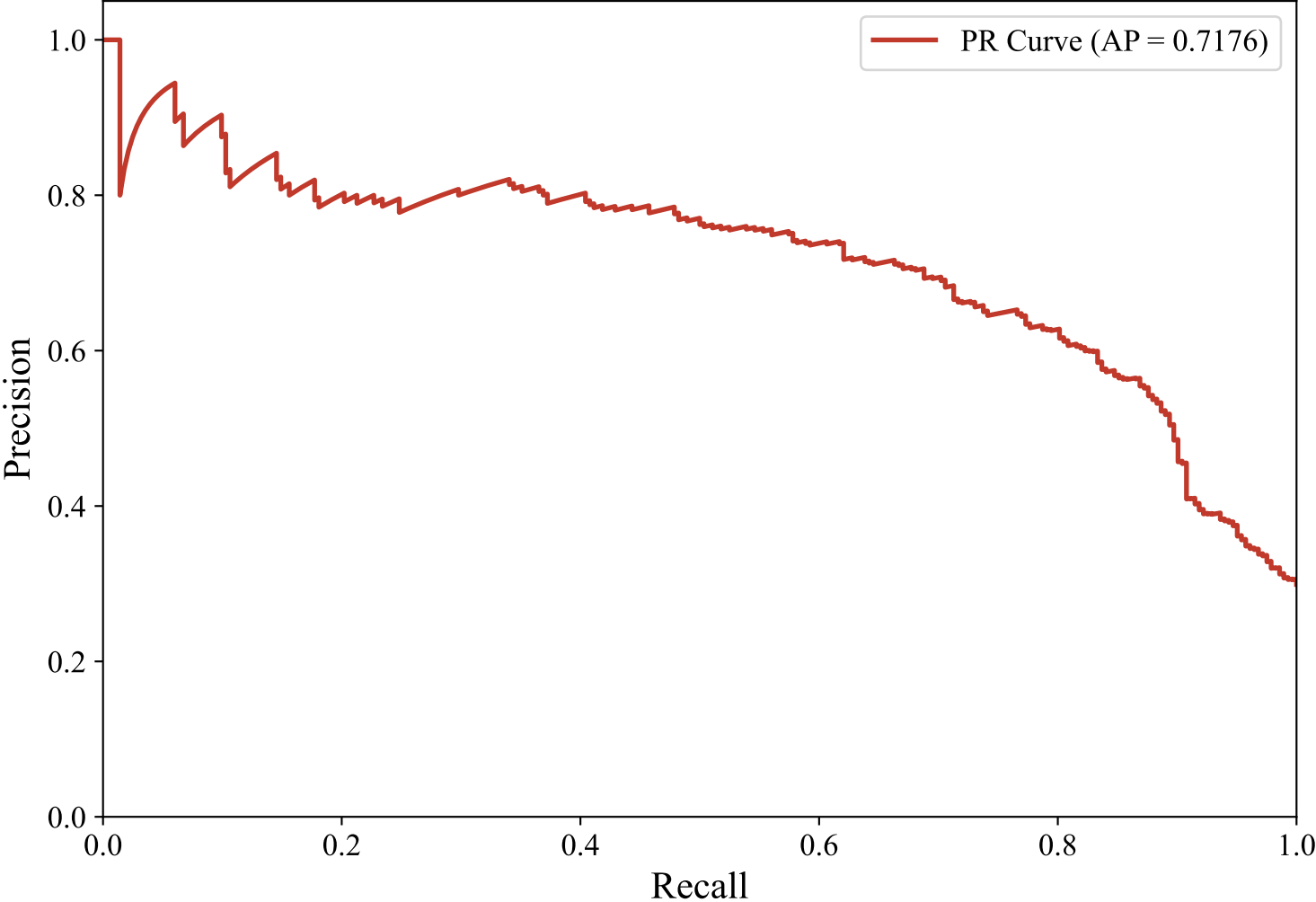
Precision-Recall Curve — ENGLISH_MANUAL (paraphrase-multilingual-MiniLM-L12-v2, Voting_Ensemble)
