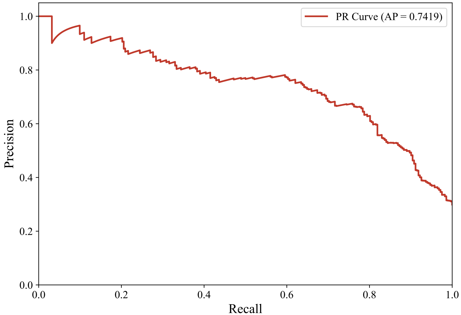
Precision-Recall Curve — ENGLISH_MANUAL (paraphrase-multilingual-MiniLM-L12-v2, XGBoost_Optimized)
