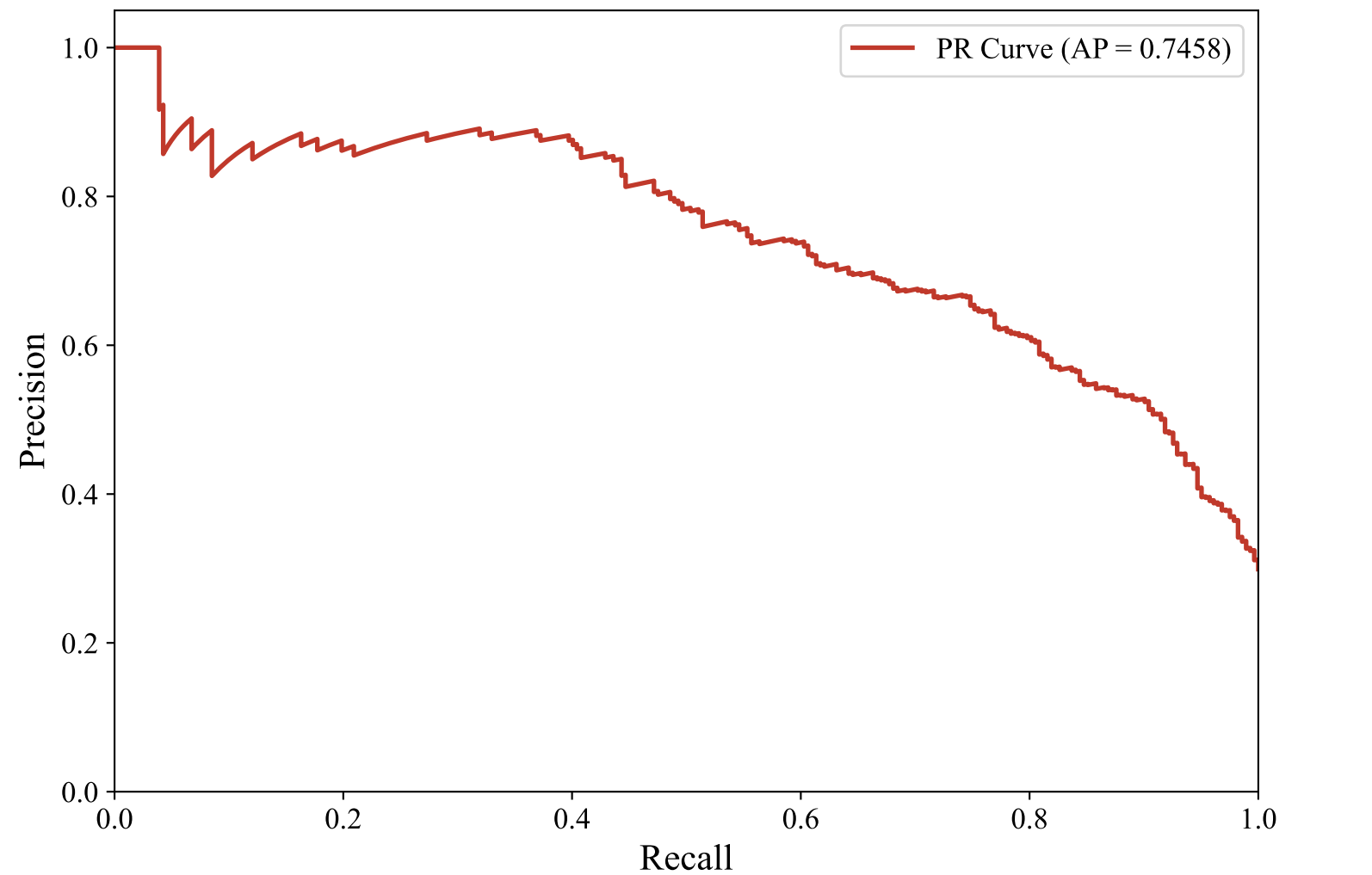
Precision-Recall Curve — ENGLISH_MANUAL (paraphrase-multilingual-mpnet-base-v2, LightGBM)
