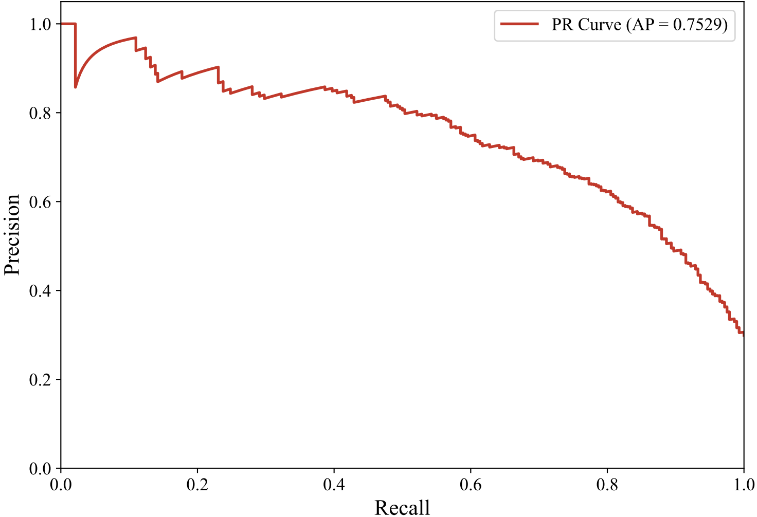
Precision-Recall Curve — ENGLISH_MANUAL (paraphrase-multilingual-mpnet-base-v2, Voting_Ensemble)
