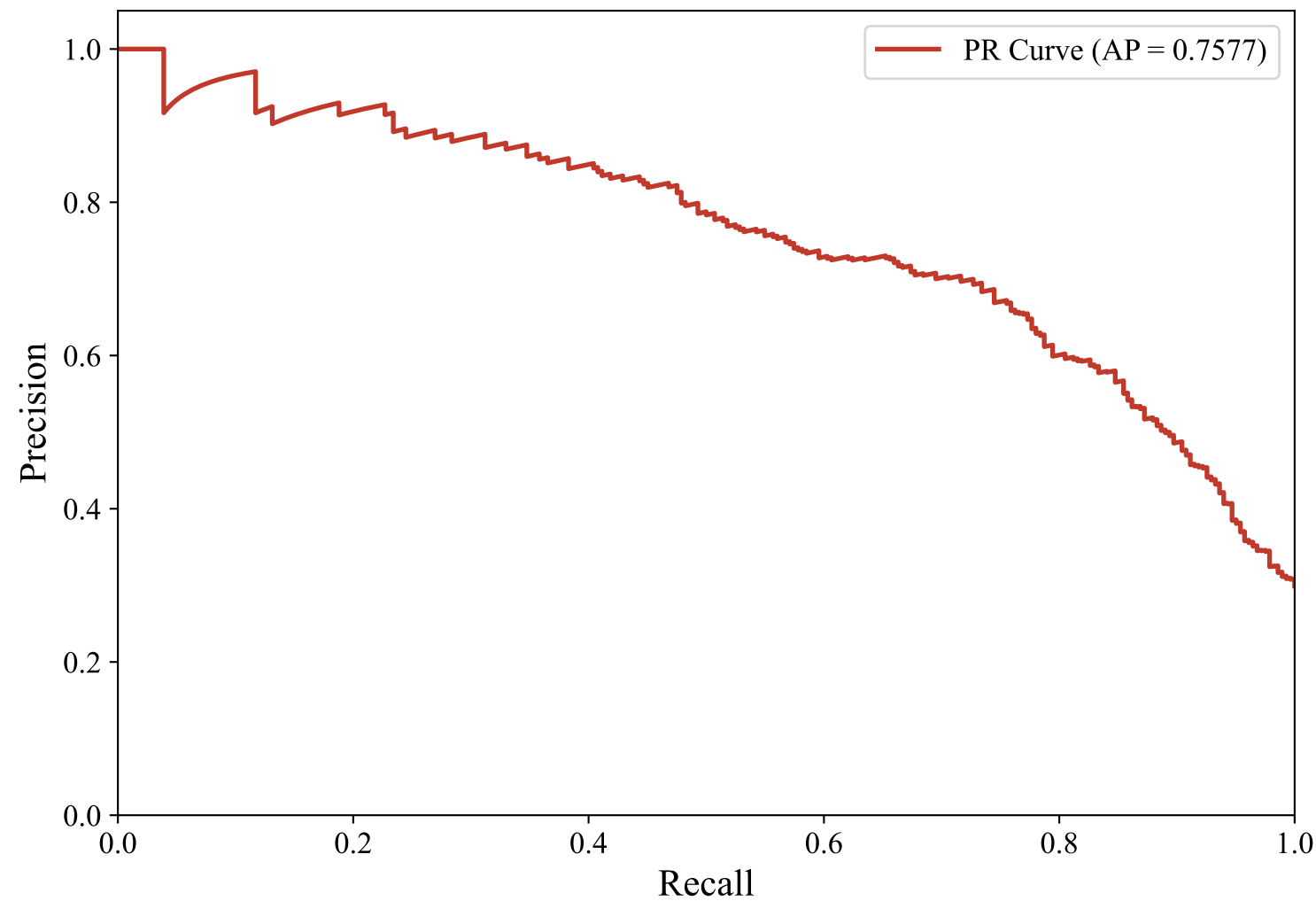
Precision-Recall Curve — ENGLISH_MANUAL (snowflake-arctic-embed-l-v2.0, XGBoost_Optimized)
