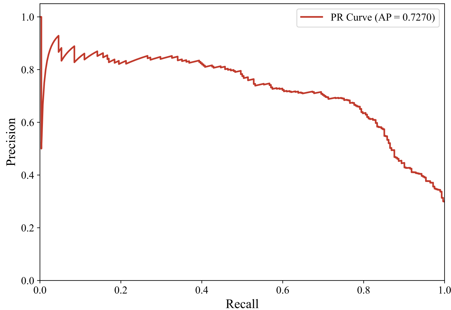
Precision-Recall Curve — ENGLISH_MANUAL (upskyy/bge-m3-korean, LightGBM)
