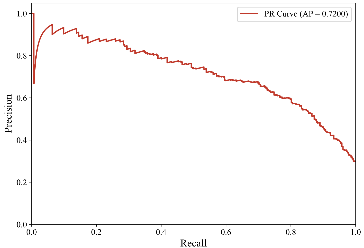
Precision-Recall Curve — ENGLISH_MANUAL (xlm-roberta-base, XGBoost_Optimized)
