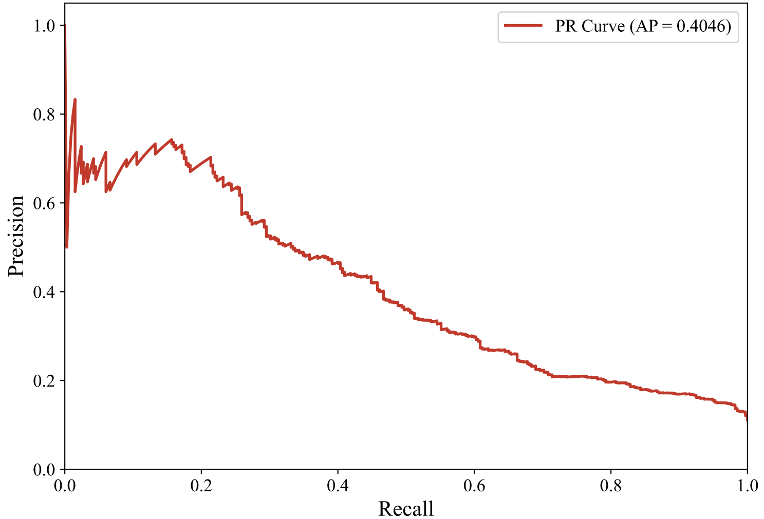
Precision-Recall Curve — GERMAN_MANUAL (bert-base-multilingual-uncased, Random_Forest)
