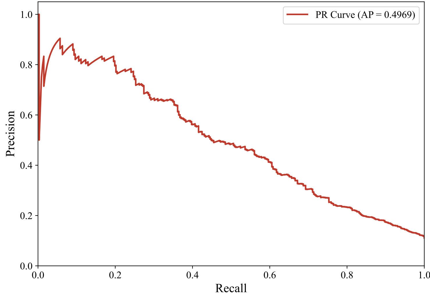
Precision-Recall Curve — GERMAN_MANUAL (bert-base-multilingual-uncased, XGBoost_Optimized)
