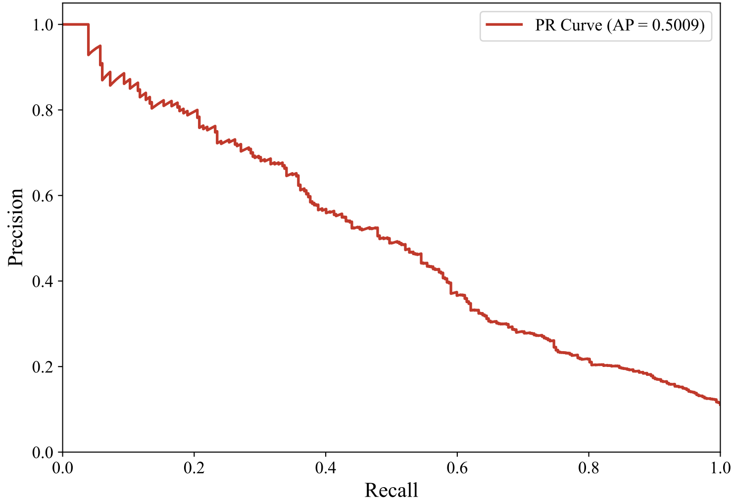
Precision-Recall Curve — GERMAN_MANUAL (efederici/e5-base-multilingual-4096, LightGBM)
