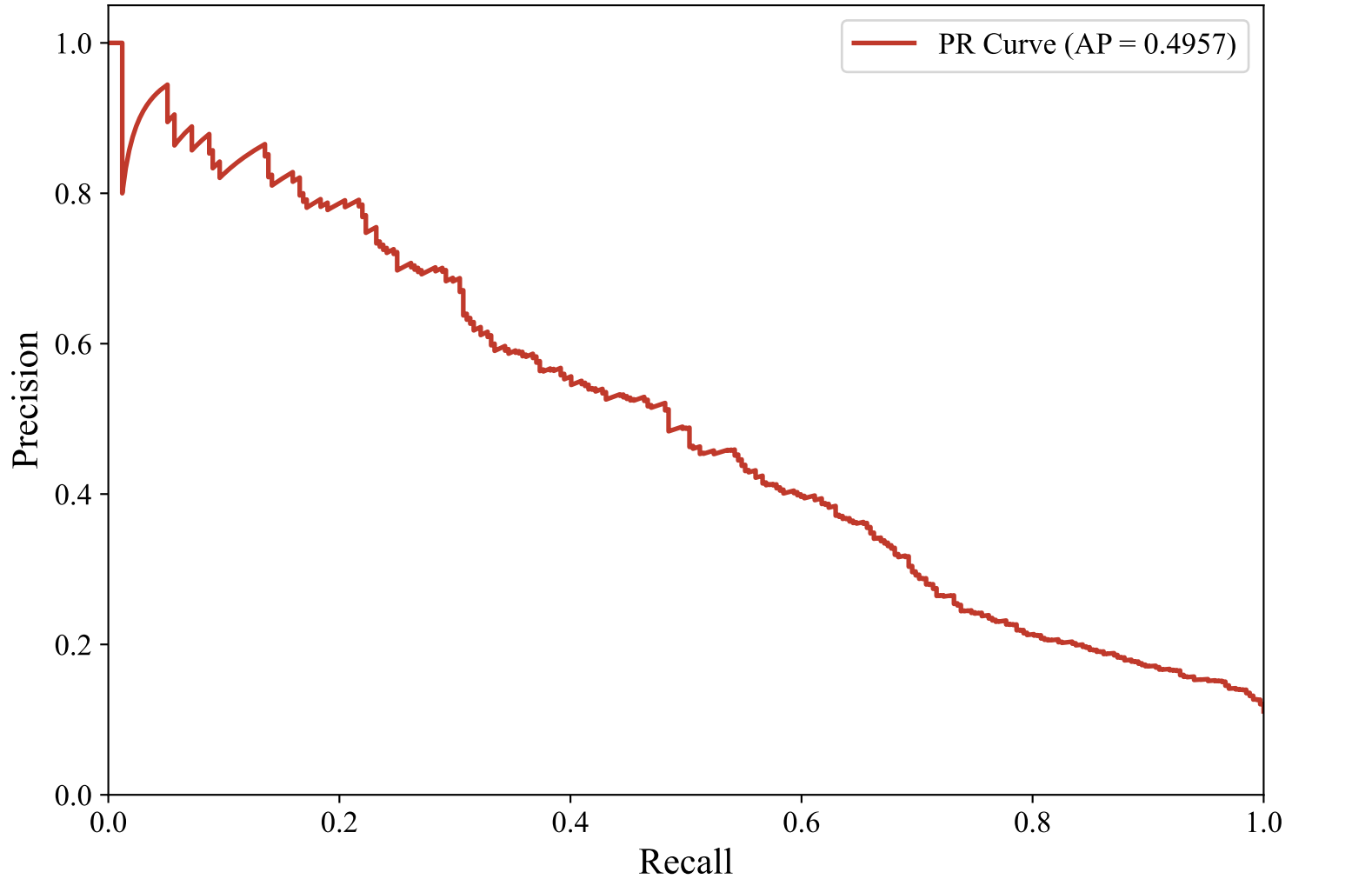
Precision-Recall Curve — GERMAN_MANUAL (efederici/e5-base-multilingual-4096, XGBoost_Optimized)
