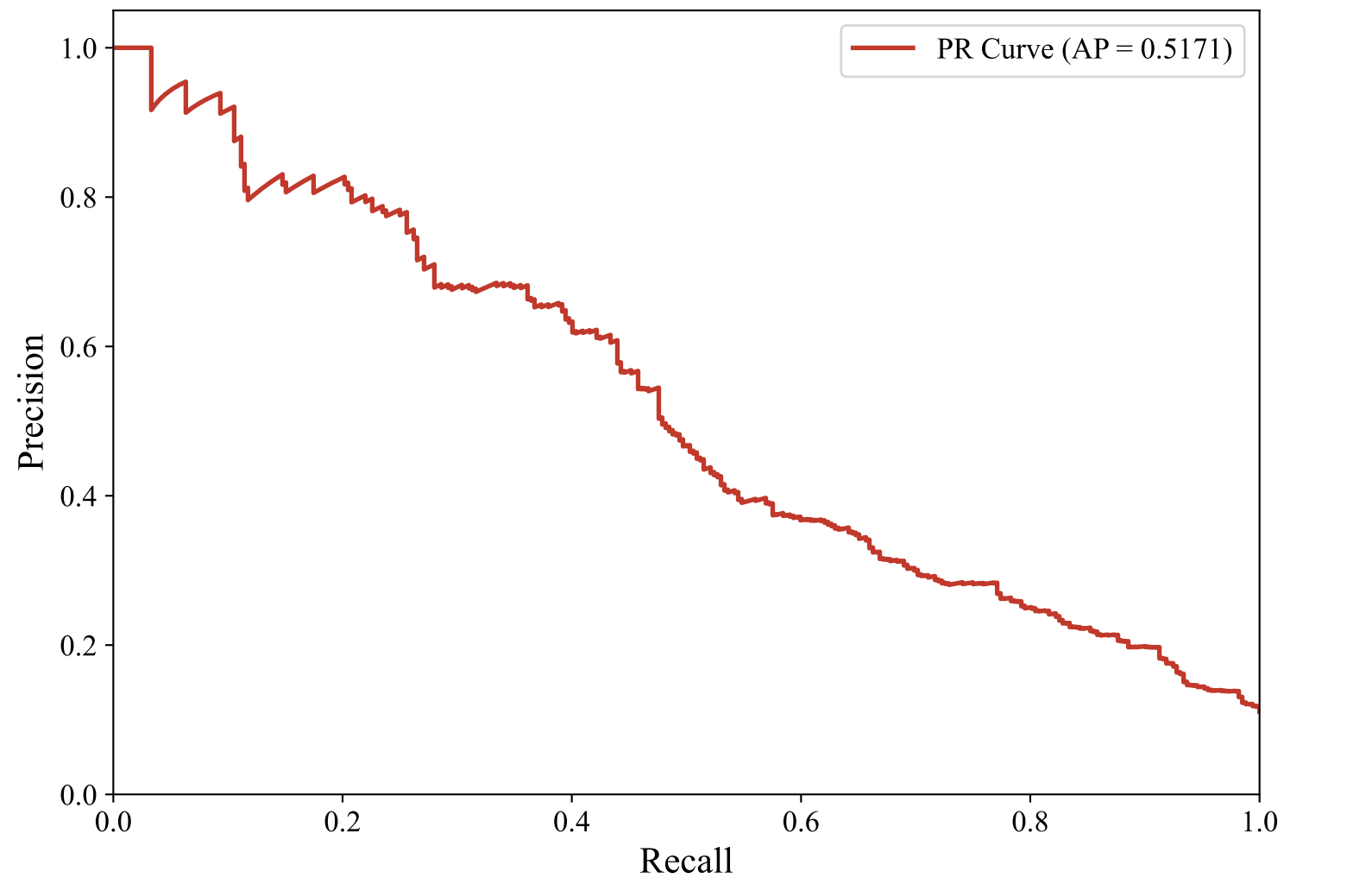
Precision-Recall Curve — GERMAN_MANUAL (intfloat/multilingual-e5-large-instruct, Random_Forest)
