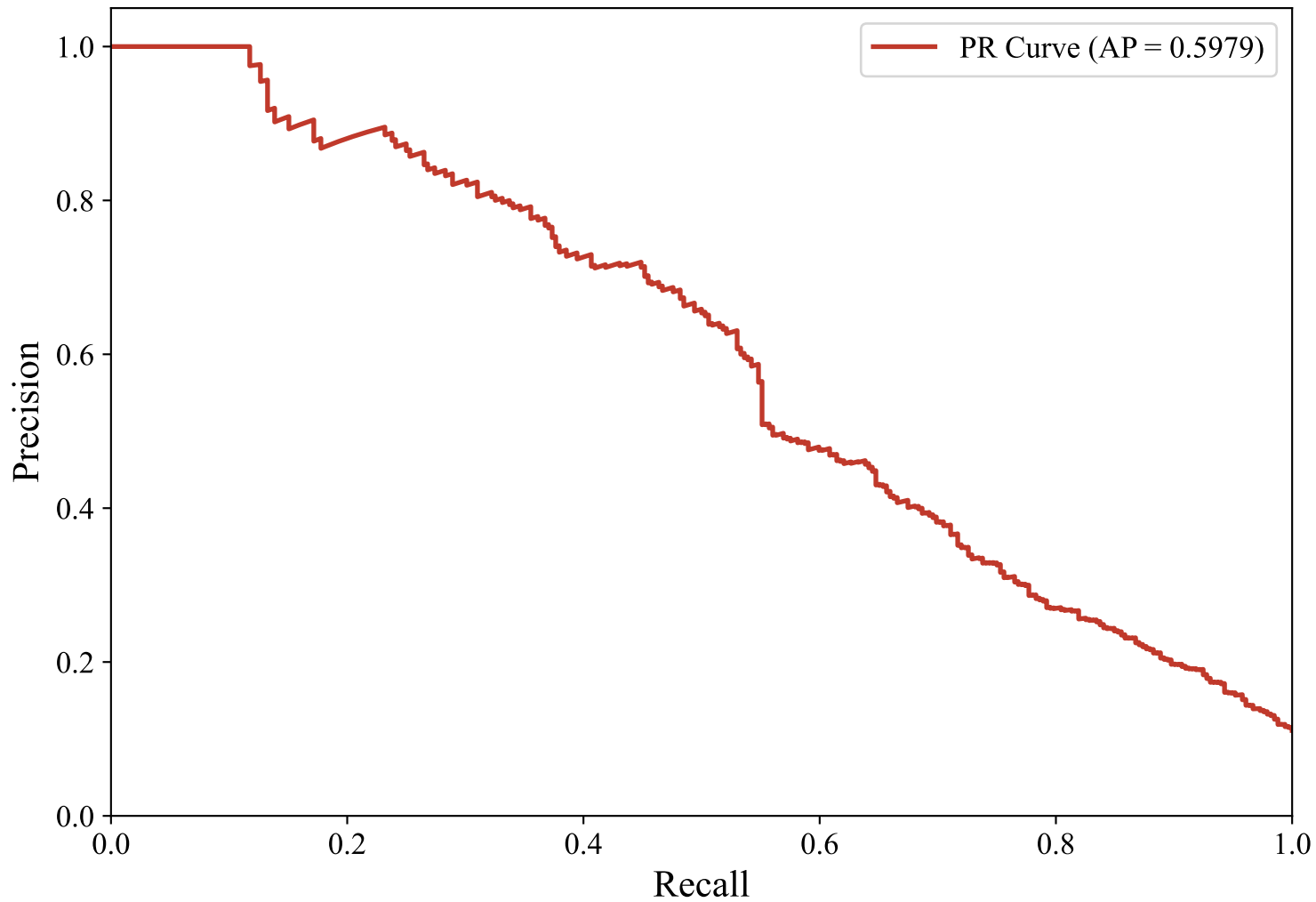
Precision-Recall Curve — GERMAN_MANUAL (intfloat/multilingual-e5-large-instruct, XGBoost_Optimized)
