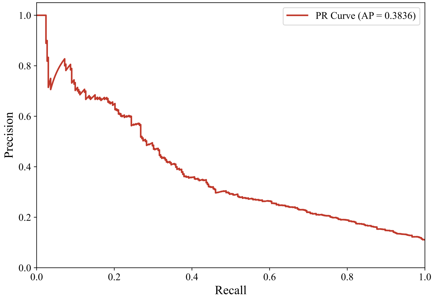
Precision-Recall Curve — GERMAN_MANUAL (paraphrase-multilingual-MiniLM-L12-v2, LightGBM_Optimized)
